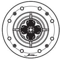
8.25" (210mm) Cut-Out Diameter Front View
